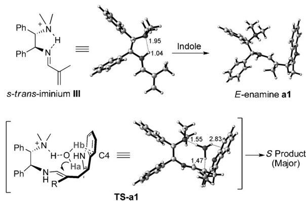
Figure 1. Calculated intermediates and transition structures for water-bridged proton transfer (only enamine a1 and TS-a1 shown).
